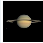
Saturn
