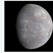
Mercury
